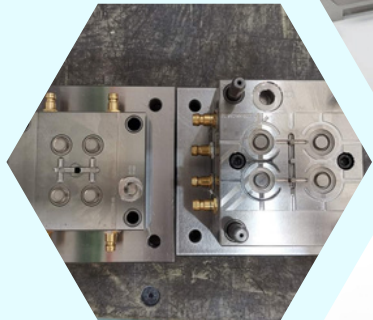
Cap Mould
